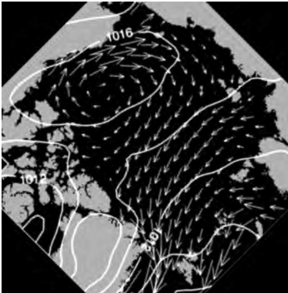
Mean Sea Ice Drift
