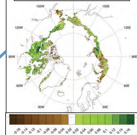
Vegetative Greenness Max-NDVI: 1999-2013
