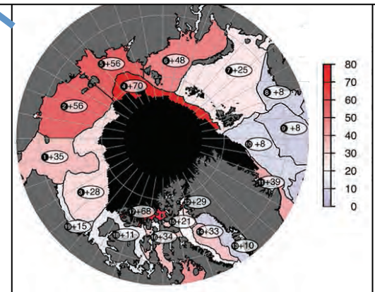
Primary Productivity Change in occurrence of double bloom (%) 1998-2001 versus 2007-2012
