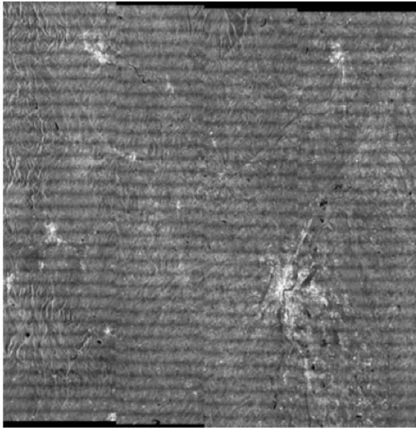
TSX-ScanSAR image
