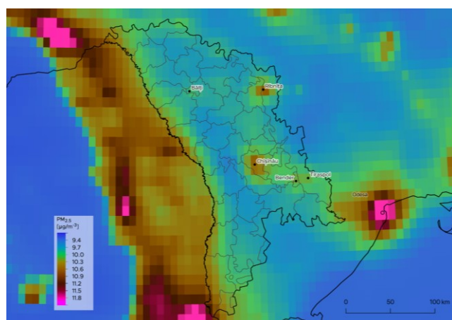
FIGURE 28 Average concentrations of PM_{2.5} over Moldova between August 2017 and July 2020 obtained from the Copernicus Atmosphere Monitoring Service data. (Contains modified Copernicus Atmosphere Monitoring Service Information [2020])
