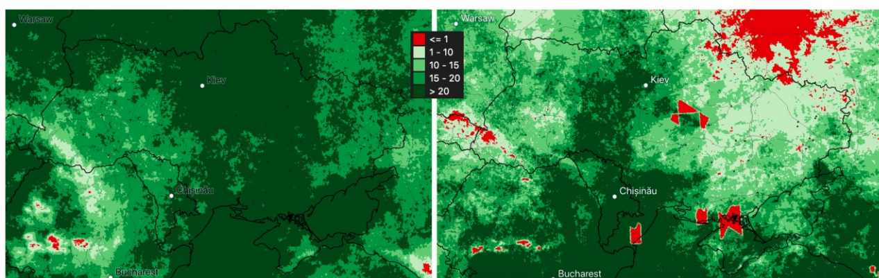
Figure 4: Comparison of valid pixels (count) from S5P satellite measurements in May 2018 (left picture) and December 2019 (right picture). Source: Contains modified Copernicus Sentinel-5p data [2019-2020] processed by WfS
