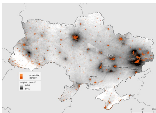
FIGURE 45 Average concentrations of nitrogen dioxide over Ukraine between May 2018 and July 2020 obtained from the Copernicus S-5p satellite data. Supplemented with population density 2019 data provided by UNDP Ukraine (Contains modified Copernicus Sentinel data and [2020])
