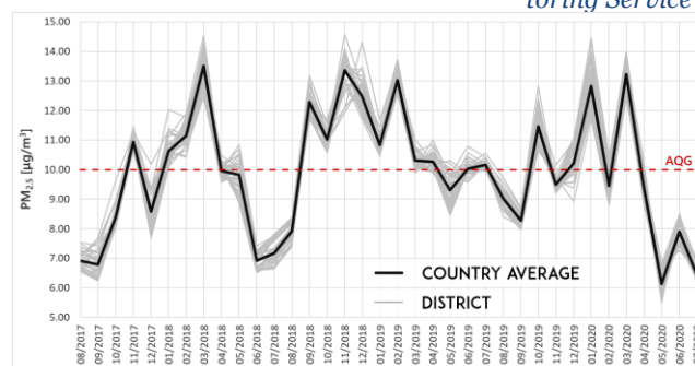
FIGURE 30 Average monthly concentrations of PM_{2.5} in the districts of Moldova between August 2017 and July 2020 obtained from the Copernicus Atmosphere Monitoring Service data. The AQG abbreviation represents the Air Quality Guideline proposed by the WHO. (Contains modified Copernicus Atmosphere Monitoring Service Information [2020])
