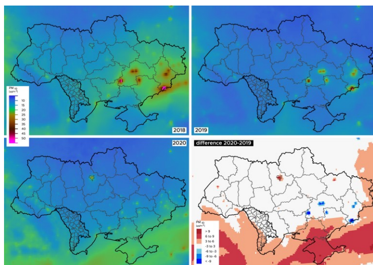
FIGURE 44 Average concentrations of particles smaller than 10 \mu\text{m} ( \text{PM}_{10} ) over Ukraine and Moldova between 17 March 2020 and 15 May 2020 compared with the same period of 2019 and 2018 obtained from the Copernicus Atmosphere Monitoring Service. (Contains modified Copernicus Atmosphere Monitoring Service Information [2020])
