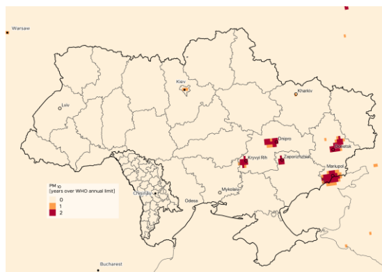
FIGURE 32 Number of years when the WHO annual limit for PM 10 was exceeded over Ukraine and Moldova between August 2017 and July 2020 obtained from the Copernicus Atmosphere Monitoring Service data. (Contains modified Copernicus Atmosphere Monitoring Service Information [2020])
