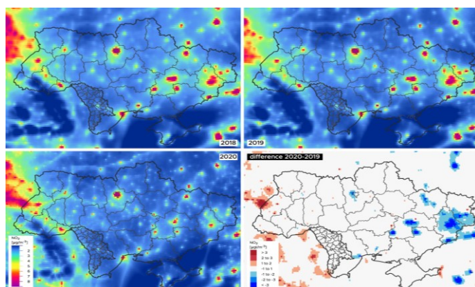
FIGURE 39 Average concentrations of nitrogen dioxide over Ukraine and Moldova between 17 March 2020 and 15 May 2020 compared with the same period of 2019 and 2018 obtained from the Copernicus Atmosphere Monitoring Service. (Contains modified Copernicus Atmosphere Monitoring Service Information [2020])
