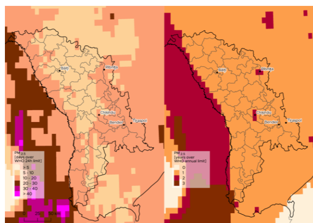
FIGURE 29 Number of days with the PM_{2.5} WHO 24-hour mean AQG value exceeded (left) and number of years with the PM_{2.5} WHO annual-mean AQG value exceeded (right) over Moldova between August 2017 and July 2020. (Contains modified Copernicus Atmosphere Monitoring Service Information [2020])
