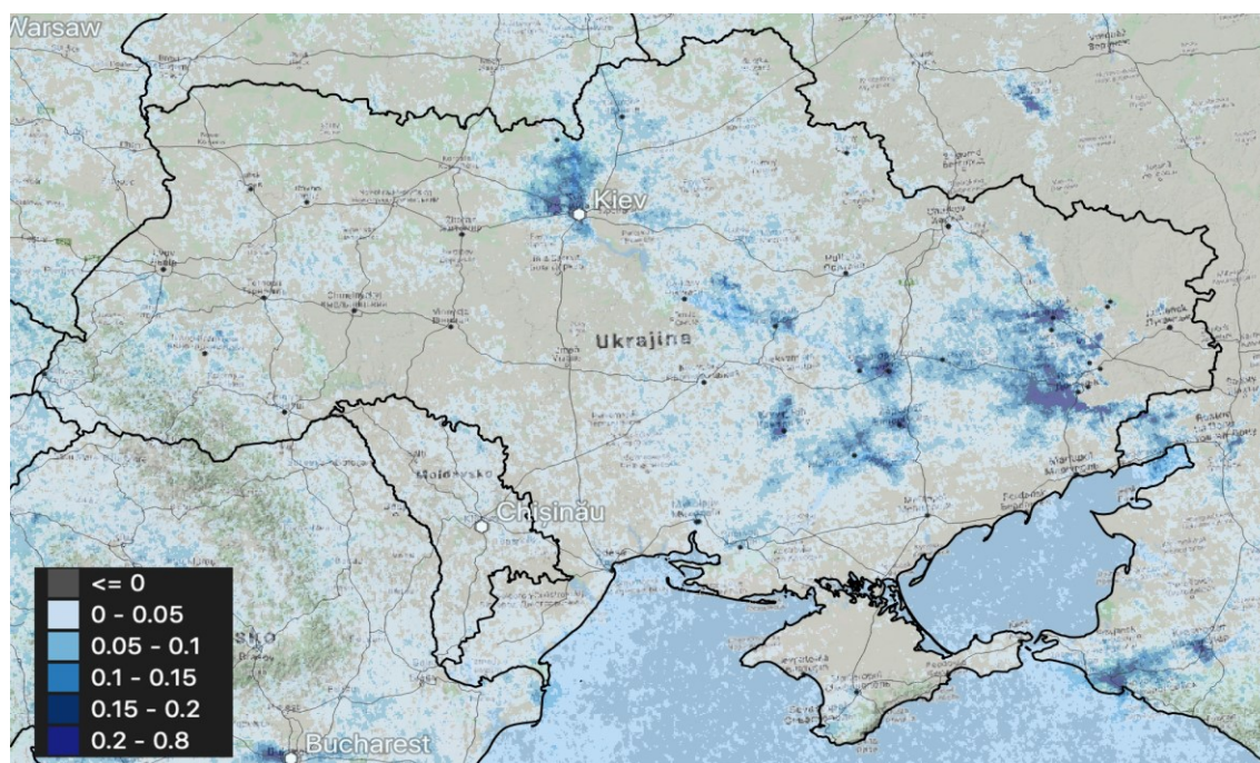
Figure 5: Decrease of NO 2 levels during the COVID-19 situation March+May 2020 in Ukraine and Moldova from S5P satellite measurements (Compare to March+May 2019) without adjustments for open fires, climatic data etc. Source: Contains modified Copernicus Sentinel-5p data [2019-2020] processed by WfS
