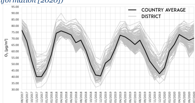
FIGURE 21 Average monthly concentrations of O 3 in the districts of Ukraine between August 2017 and July 2020 obtained from the Copernicus Atmosphere Monitoring Service data. (Contains modified Copernicus Atmosphere Monitoring Service Information [2020])
