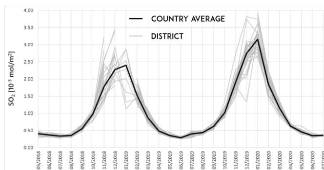
FIGURE 16 Average monthly concentrations of sulfur dioxide in the districts of Moldova between May 2018 and July 2020 obtained from the Copernicus S-5p satellite data. (Contains modified Copernicus Sentinel data [2020])
