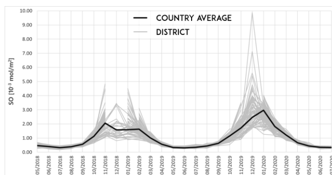
FIGURE 14 Average monthly concentrations of sulfur dioxide in the districts of Ukraine between May 2018 and July 2020 obtained from the Copernicus S-5p satellite data. (Contains modified Copernicus Sentinel data [2020])
