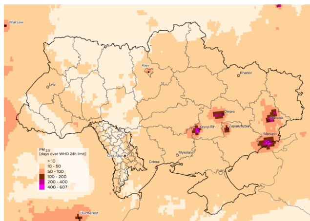
FIGURE 25 Number of days with the \text{PM}_{2.5} WHO 24-hour AQG value exceeded in Ukraine and Moldova between August 2017 and July 2020 (Contains modified Copernicus Atmosphere Monitoring Service Information [2020])
