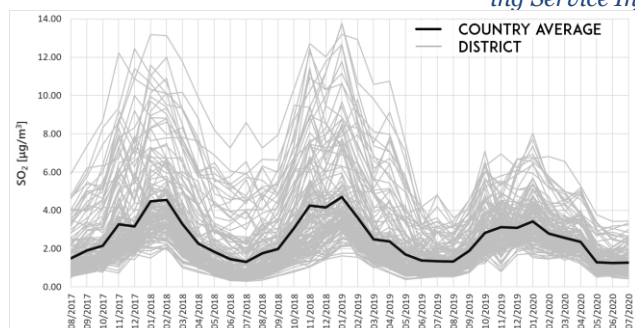
FIGURE 18 Average monthly concentrations of sulfur dioxide in the districts of Ukraine between August 2017 and July 2020 obtained from the Copernicus Atmosphere Monitoring Service data. (Contains modified Copernicus Atmosphere Monitoring Service Information [2020])
