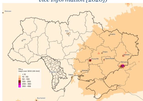
FIGURE 33 Number of days when the WHO 24-hour limit for PM 10 was exceeded over Ukraine and Moldova between August 2017 and July 2020 obtained from the Copernicus Atmosphere Monitoring Service data. (Contains modified Copernicus Atmosphere Monitoring Service Information [2020])
