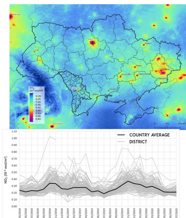
FIGURE 2 concentration of NO 2 over Ukraine from S-5p data
