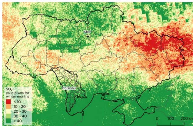
FIGURE 12 Count of valid SO 2 for winter season months of 2018/2019 and 2019/2020 over Ukraine and Moldova obtained from the Copernicus S-5p satellite data. (Contains modified Copernicus Sentinel data [2020])
