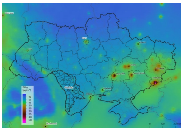
FIGURE 31 Average concentrations of particles smaller than 10 µm (PM 10 ) in the districts of Ukraine between August 2017 and July 2020 obtained from the Copernicus Atmosphere Monitoring Service data. (Contains modified Copernicus Atmosphere Monitoring Service Information [2020])
