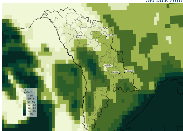
FIGURE 22 Mean concentrations of O 3 over Moldova between August 2017 and July 2020 obtained from the Copernicus Atmosphere Monitoring Service data. (Contains modified Copernicus Atmosphere Monitoring Service Information [2020])
