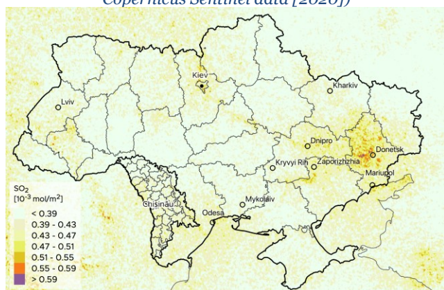
FIGURE 13 Median concentrations of SO 2 over Ukraine and Moldova between May 2018 and July 2020 obtained from the Copernicus S-5p satellite data. (Contains modified Copernicus Sentinel data [2020])
