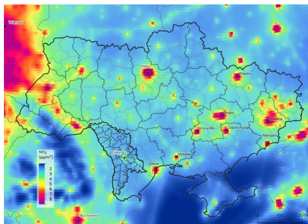
Figure 1. Average concentrations of NO 2 in Ukraine and Moldova between August 2017 and July 2020 obtained from the CAMS data. (Contains modified Copernicus Atmosphere Monitoring Service Information [2020])
