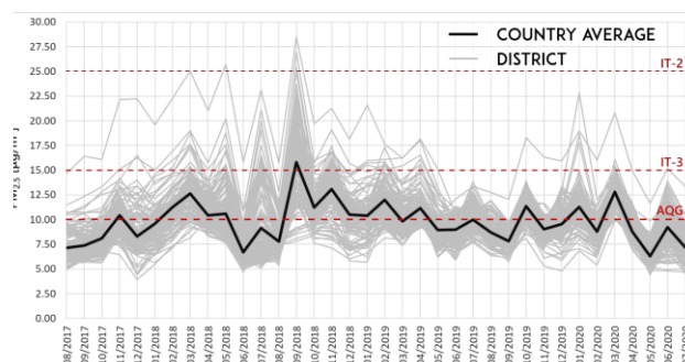
FIGURE 27 Average monthly concentrations of particles smaller than 2.5\ \mu\text{m} ( \text{PM}_{2.5} ) in the districts of Ukraine between August 2017 and July 2020 obtained from the Copernicus Atmosphere Monitoring Service data. The AQG, IT-3, and IT-2 abbreviations represent the Air Quality Guideline, Interim Target 3, and Interim Target 2, respectively, all proposed by the WHO. (Contains modified Copernicus Atmosphere Monitoring Service Information [2020])
