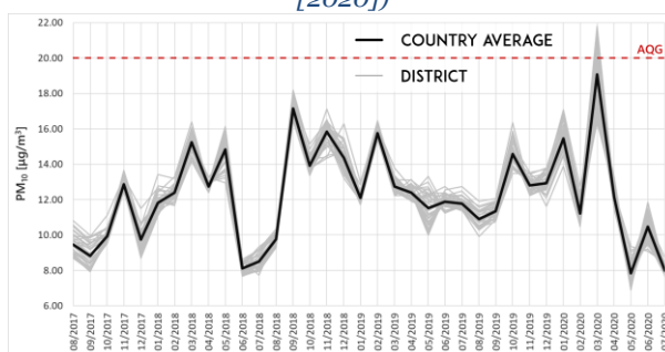
FIGURE 36 Average monthly concentrations of PM 10 in the districts of Moldova between August 2017 and July 2020 obtained from the Copernicus Atmosphere Monitoring Service data. The AQG abbreviation represents the Air Quality Guideline proposed by the WHO. (Contains modified Copernicus Atmosphere Monitoring Service Information [2020])
