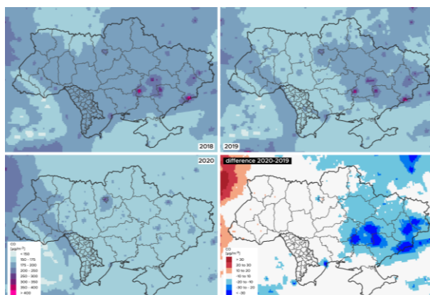
FIGURE 40 Average concentrations of carbon monoxide over Ukraine and Moldova between 17 March 2020 and 15 May 2020 compared with the same period of 2019 and 2018 obtained from the Copernicus Atmosphere Monitoring Service. (Contains modified Copernicus Atmosphere Monitoring Service Information [2020])
