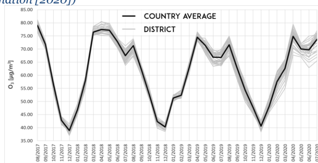
FIGURE 23 Average monthly concentrations of ozone in the districts of Moldova between August 2017 and July 2020 obtained from the Copernicus Atmosphere Monitoring Service data. (Contains modified Copernicus Atmosphere Monitoring Service Information [2020])
