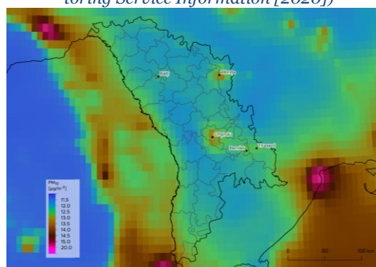
FIGURE 35 Average concentrations of PM 10 over Moldova between August 2017 and July 2020 obtained from the Copernicus Atmosphere Monitoring Service data. (Contains modified Copernicus Atmosphere Monitoring Service Information [2020])
