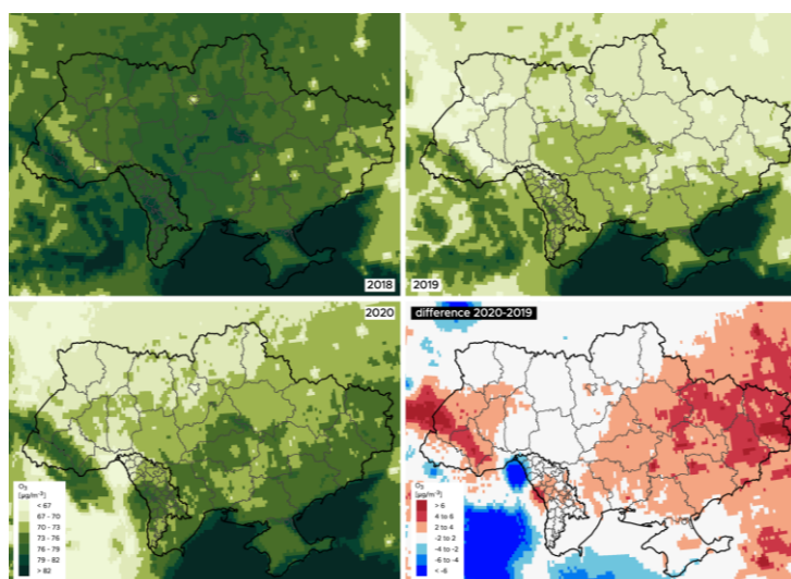
FIGURE 42 Average concentrations of ozone over Ukraine and Moldova between 17 March 2020 and 15 May 2020 compared with the same period of 2019 and 2018 obtained from the Copernicus Atmosphere Monitoring Service. (Contains modified Copernicus Atmosphere Monitoring Service Information [2020])
