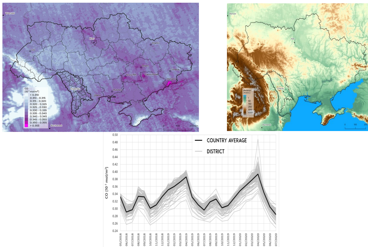
FIGURE 6 Carbon monoxide CO in Ukraine (S-5p)
