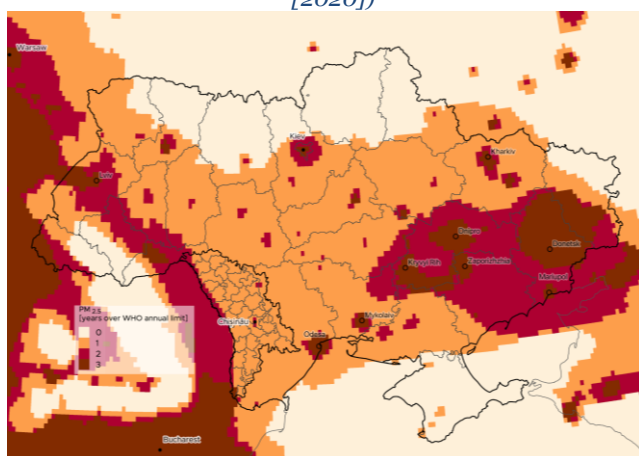
FIGURE 26 Number of years when the WHO annual limit for \text{PM}_{2.5} was exceeded over Ukraine and Moldova between August 2017 and July 2020. (Contains modified Copernicus Atmosphere Monitoring Service Information [2020])
