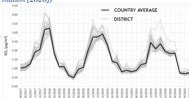
FIGURE 19 Average monthly concentrations of sulfur dioxide in the districts of Moldova between August 2017 and July 2020 obtained from the Copernicus Atmosphere Monitoring Service data. (Contains modified Copernicus Atmosphere Monitoring Service Information [2020])
