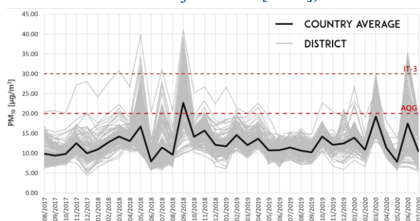
FIGURE 34 Average monthly concentrations of particles smaller than 10 µm (PM 10 ) in the districts of Ukraine between August 2017 and July 2020 obtained from the Copernicus Atmosphere Monitoring Service data. The AQG and IT-3 abbreviations represent the Air Quality Guideline and the Interim Target 3, respectively, both proposed by the WHO. (Contains modified Copernicus Atmosphere Monitoring Service Information [2020])
