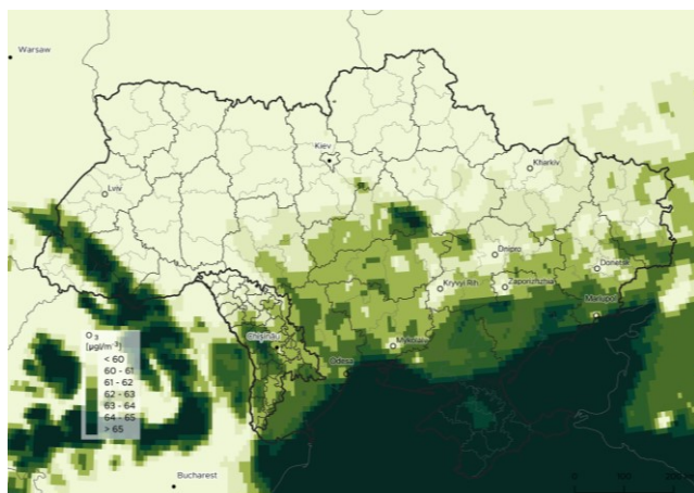
FIGURE 20 Average concentrations of O 3 over Ukraine and Moldova between August 2017 and July 2020 obtained from the Copernicus Atmosphere Monitoring Service data. (Contains modified Copernicus Atmosphere Monitoring Service Information [2020])
