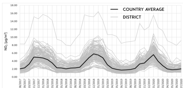
FIGURE 4 Average monthly concentrations of NO 2 in the districts of Ukraine between August 2017 and July 2020 obtained from the CAMS data. (Contains modified Copernicus Atmosphere Monitoring Service Information [2020])
