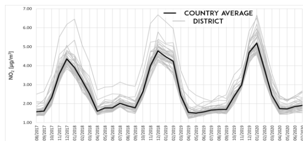
FIGURE 5 Average monthly concentrations of nitrogen dioxide in the districts of Moldova between August 2017 and July 2020 obtained from the Copernicus Atmosphere Monitoring Service data. (Contains modified Copernicus Atmosphere Monitoring Service Information [2020])
