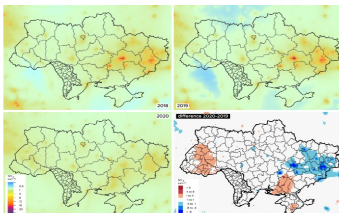
FIGURE 41 Average concentrations of sulfur dioxide over Ukraine and Moldova between 17 March 2020 and 15 May 2020 compared with the same period of 2019 and 2018 obtained from the Copernicus Atmosphere Monitoring Service. (Contains modified Copernicus Atmosphere Monitoring Service Information [2020])
