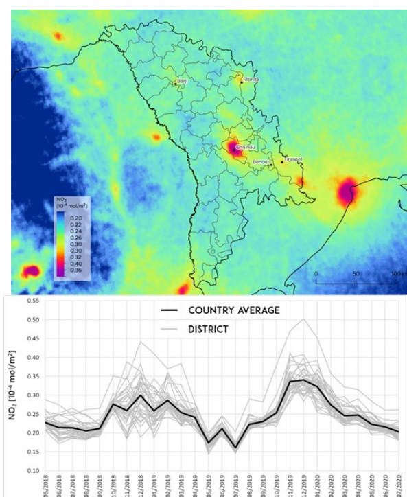
FIGURE 3 concentration of NO 2 over Moldova from S-5p data
