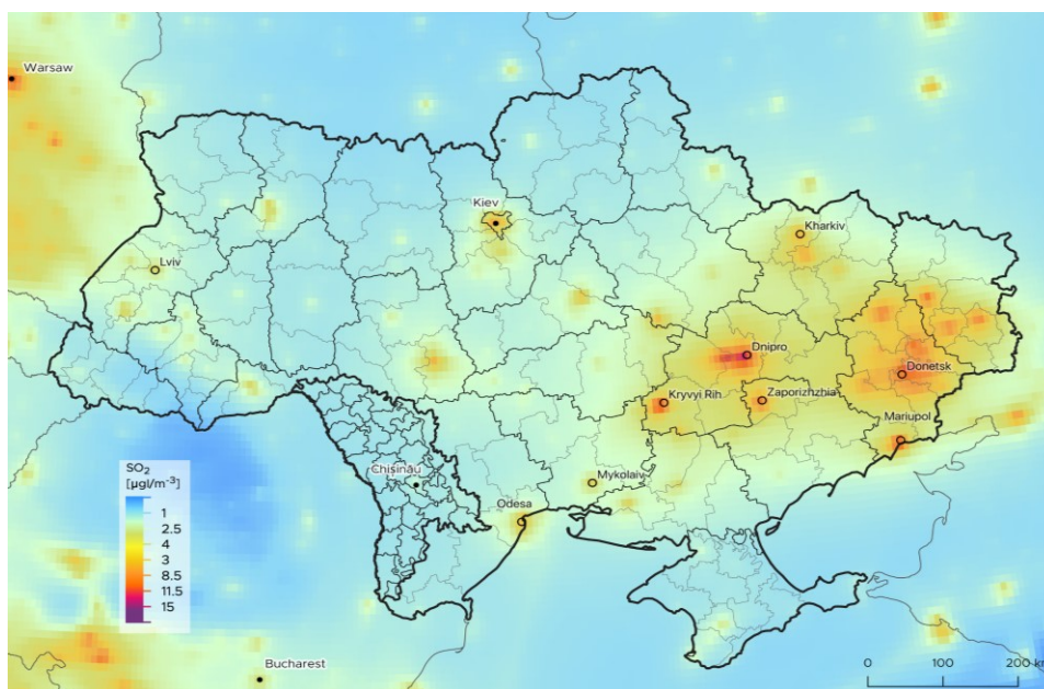
FIGURE 17 Average concentrations of sulfur dioxide over Ukraine and Moldova between August 2017 and July 2020 obtained from the Copernicus Atmosphere Monitoring Service data. (Contains modified Copernicus Atmosphere Monitoring Service Information [2020])
