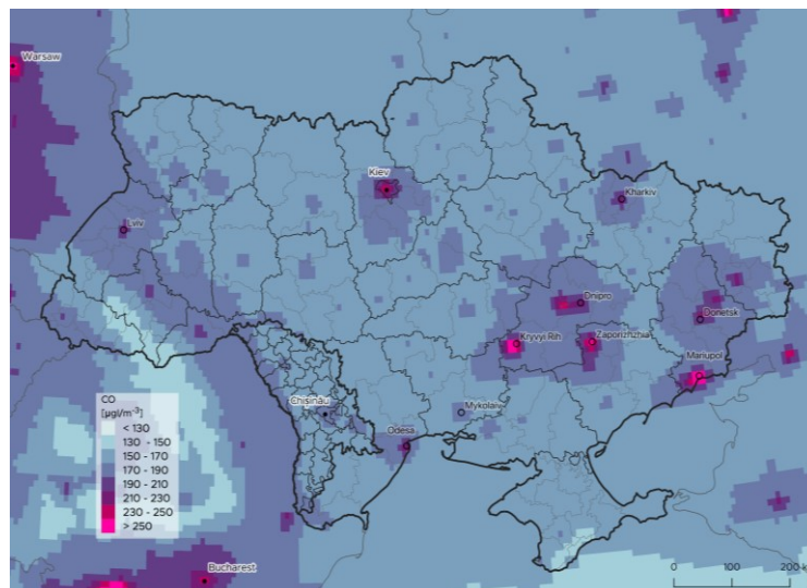
FIGURE 8 Average concentrations of carbon monoxide over Ukraine and Moldova between August 2017 and July 2020 obtained from the Copernicus Atmosphere Monitoring Service data. (Contains modified Copernicus Atmosphere Monitoring Service Information [2020])
