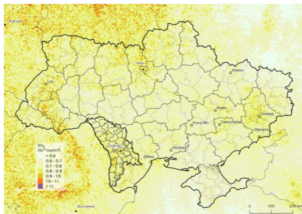
FIGURE 11 Average concentrations of SO 2 over Ukraine and Moldova between May 2018 and July 2020 obtained from the Copernicus S-5p satellite data. (Contains modified Copernicus Sentinel data [2020])
