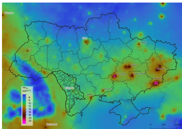
FIGURE 24 Average concentrations of particles smaller than 2.5\ \mu\text{m} ( \text{PM}_{2.5} ) in the districts of Ukraine between August 2017 and July 2020 obtained from the Copernicus Atmosphere Monitoring Service data. (Contains modified Copernicus Atmosphere Monitoring Service Information [2020])
