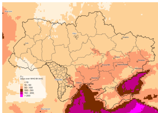
Figure 1. Number of days when the WHO 8-hour limit for O 3 was exceeded over Ukraine and Moldova between August 2017 and July 2020. (Contains modified Copernicus Atmosphere Monitoring Service Information [2020])
