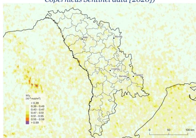
FIGURE 15 Median values of overall concentrations of SO 2 over Moldova between May 2018 and July 2020 obtained from the Copernicus S-5p satellite data. (Contains modified Copernicus Sentinel data [2020])
