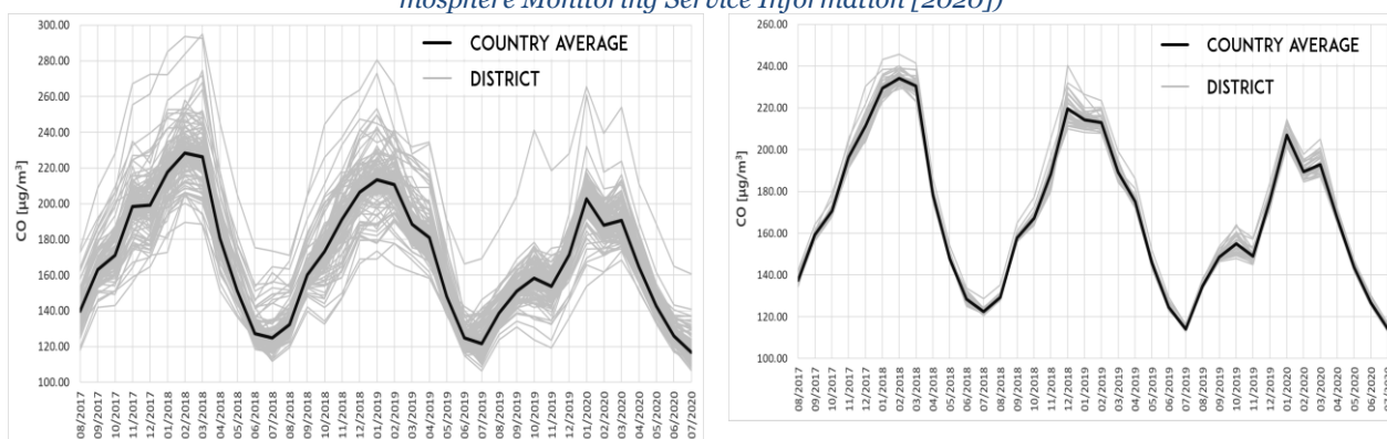
FIGURE 10 Average monthly concentrations of carbon monoxide in the districts of Moldova between August 2017 and July 2020 obtained from the Copernicus Atmosphere Monitoring Service data. (Contains modified Copernicus Atmosphere Monitoring Service Information [2020])
