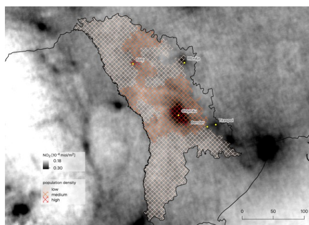
FIGURE 46 Average concentrations of nitrogen dioxide over Moldova between May 2018 and July 2020 obtained from the Copernicus S-5p satellite data. Supplemented with population density 2019 data provided by UNDP Moldova (Contains modified Copernicus Sentinel data and [2020])
