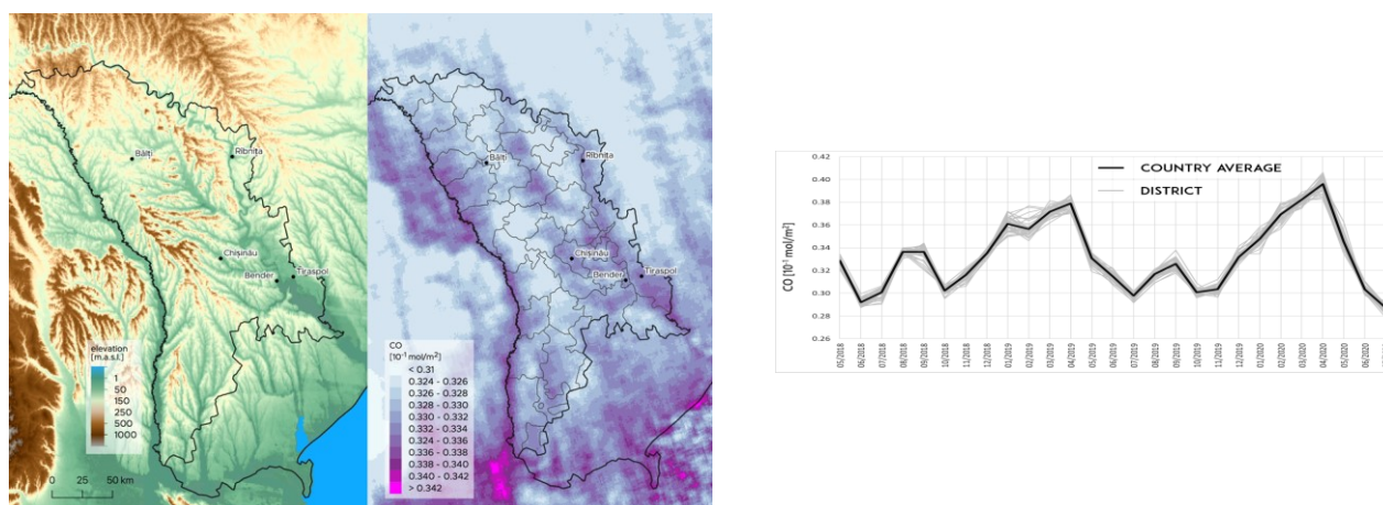
FIGURE 7 Carbon monoxide CO in Moldova (S-5p)
